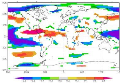
Figure 4: Linear correlations between July Surface U in the Caribbean (Predictor 1) and August-October sea surface temperature (panel a), August-October sea level pressure (panel b), August-October 850 mb zonal wind (panel c) and August-October 200 mb zonal wind (panel d) over the period from 1979-2011.
