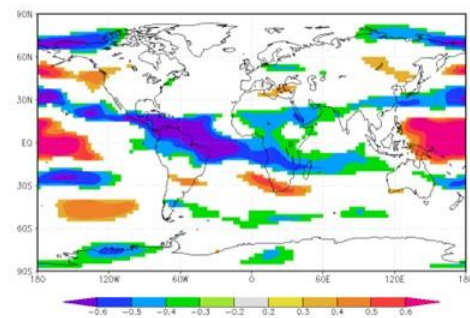
Figure 4: Linear correlations between July Surface U in the Caribbean (Predictor 1) and August-October sea surface temperature (panel a), August-October sea level pressure (panel b), August-October 850 mb zonal wind (panel c) and August-October 200 mb zonal wind (panel d) over the period from 1979-2011.
