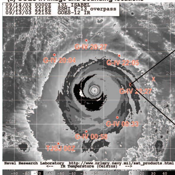
FIG. 6. (a) GOES infrared satellite imagery at 2215 UTC (courtesy of NRL/Monterey) showing extent of hurricane outflow, and the dropwindsonde profile locations (red dots with UTC time labels) used in the outflow temperature calculation; "x" indicates location of additional outflow jet sample at 553-km radius from center. (b) High-altitude wind speed ( \text{m s}^{-1} ) and \theta_e (K) from NOAA Gulfstream-IV dropwindsonde at 341-km radius from center at 2227 UTC. Tangential (red) and radial (blue) winds show anticyclonic outflow, with \theta_e in green. Black dashed line indicates linearly interpolated data.
