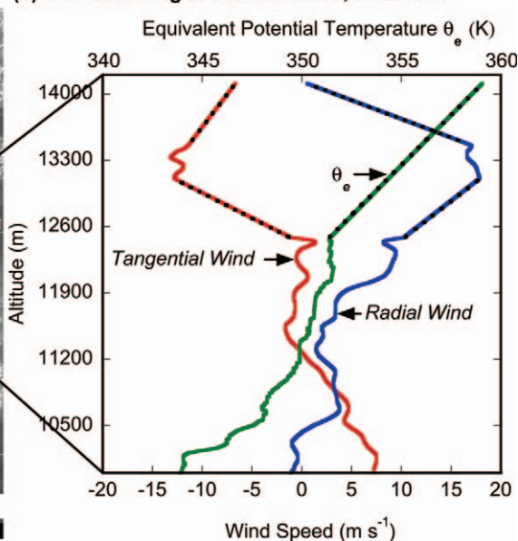
FIG. 6. (a) GOES infrared satellite imagery at 2215 UTC (courtesy of NRL/Monterey) showing extent of hurricane outflow, and the dropwindsonde profile locations (red dots with UTC time labels) used in the outflow temperature calculation; "x" indicates location of additional outflow jet sample at 553-km radius from center. (b) High-altitude wind speed ( \text{m s}^{-1} ) and \theta_e (K) from NOAA Gulfstream-IV dropwindsonde at 341-km radius from center at 2227 UTC. Tangential (red) and radial (blue) winds show anticyclonic outflow, with \theta_e in green. Black dashed line indicates linearly interpolated data.
